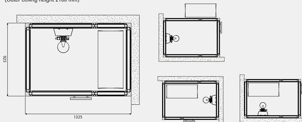
Tylö steam shower i130 (Outer ceiling height 2100 mm)
