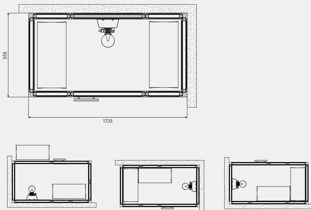
Tylö steam shower i170 (Outer ceiling height 2100 mm)
